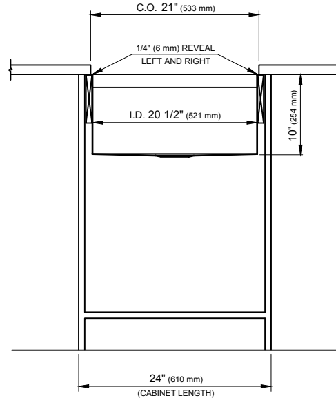
COUNTERTOP CUTOUT PLAN
