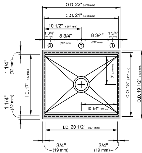
COUNTERTOP CUTOUT PLAN
